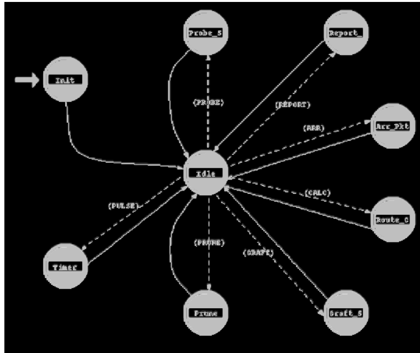
Figure 11. DVMRP process on routers
